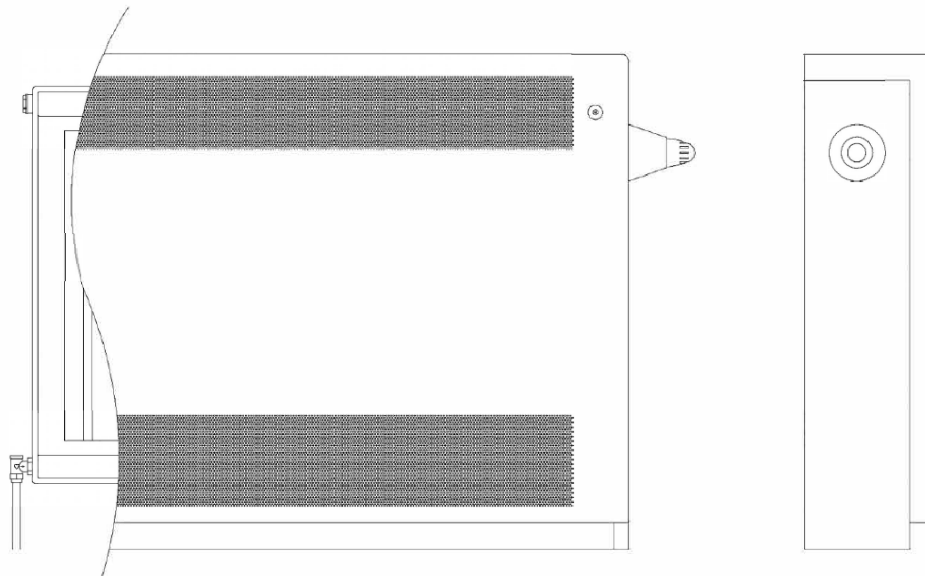
Front Elevation and Profile Shown With Anti-Ligature TRV Kit & Shroud 9213-63 in Position
